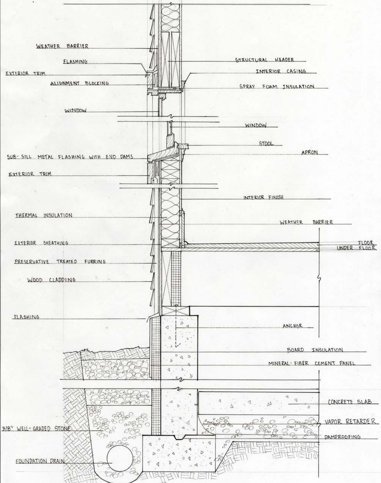
A TYPICAL FOUNDATION TO WALL CONNECTION 1 1/2" = 1'-0"
